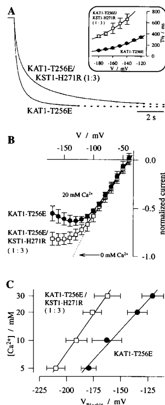
FIGURE 4 Co-expression of the Ca^{2+} -sensitive KAT1-T256E and the Ca^{2+} -insensitive KST1-H271R. At pH 5.6 KST1-H271R activates more negatively than -180 mV (Hoth et al., 1997). Each data point represents the mean of five measurements \pm standard error of the mean. (A) Co-expression slows activation kinetics of KAT1-T256E. Representative K^+ currents mediated by KAT1-T256E and KAT1-T256E/KST1-H271R mixtures (1:3). Currents were evoked by activation pulses to -150 mV starting from a holding potential of -30 mV. Current amplitudes were normalized to the steady-state value of -2.2 \mu A for KAT1-T256E and -2.4 \mu A for the KAT1-T256E/KST1-H271R mixture (1:3). Inset : Comparison of the voltage-dependence of the half-activation time ( T_{1/2} ). Solid lines represent best fits with an exponential function. (B) Co-expression reduces the Ca^{2+} sensitivity of KAT1-T256E. Tail currents recorded in 20 mM Ca^{2+} for KAT1-T256E (closed circles) and KAT1-T256E/KST1-H271R (1:3, open squares) after an activating pre-pulse to -150 mV are superimposed. The dotted line represents tail currents through KAT1-T256E and KAT1-T256E/KST1-H271R in the absence of Ca^{2+} ions, and solid lines represent best fits according to the Woodhull model (Woodhull, 1973). (C) Concentration- and voltage-dependence of the Ca^{2+} block. Half-blocking voltages ( V_{Block 1/2} ) were determined in different Ca^{2+} concentrations (5, 10, 20, and 30 mM). Note the logarithmic scale of the concentration axis.
